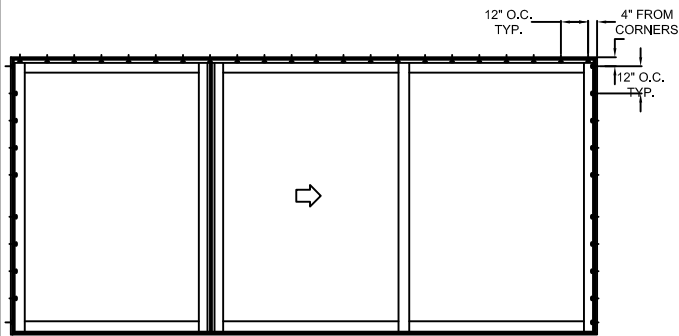
TYPICAL ELEVATION WITH FASTENER SPACING
